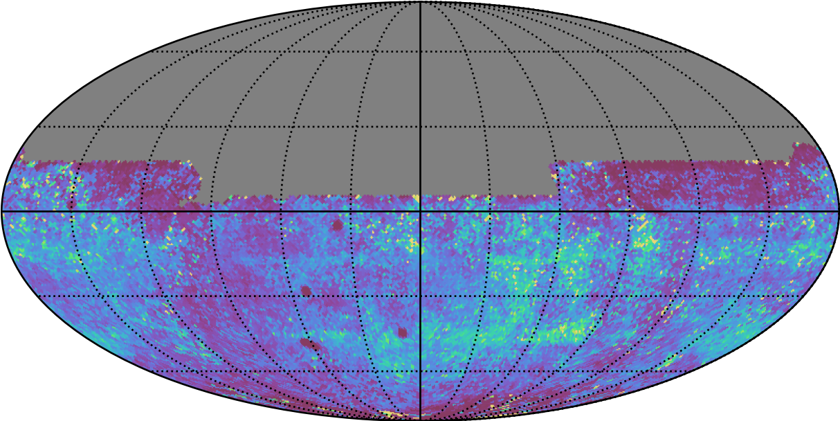
too_elab_r256_d2_gz_v3.4_10yrs All sky y band: 75th Percentile Intranight Timespan
