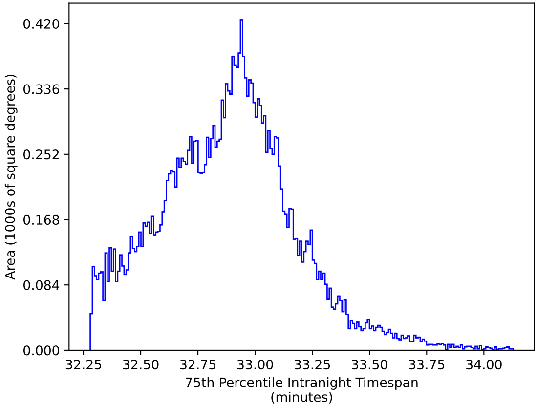
too_elab_r256_d2_gz_v3.4_10yrs All sky y band: 75th Percentile Intranight Timespan
