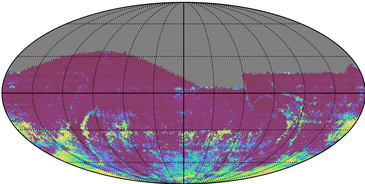
too_elab_r256_d2_gz_v3.4_10yrs All sky r band: 75th Percentile Intranight Timespan
