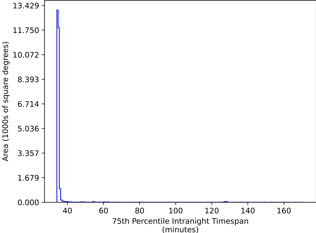
too_elab_r256_d2_gz_v3.4_10yrs All sky iz bands: 75th Percentile Intranight Timespan
