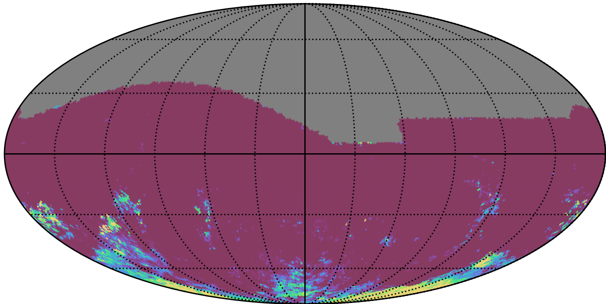
too_elab_r256_d2_gz_v3.4_10yrs All sky gr bands: 75th Percentile Intranight Timespan
