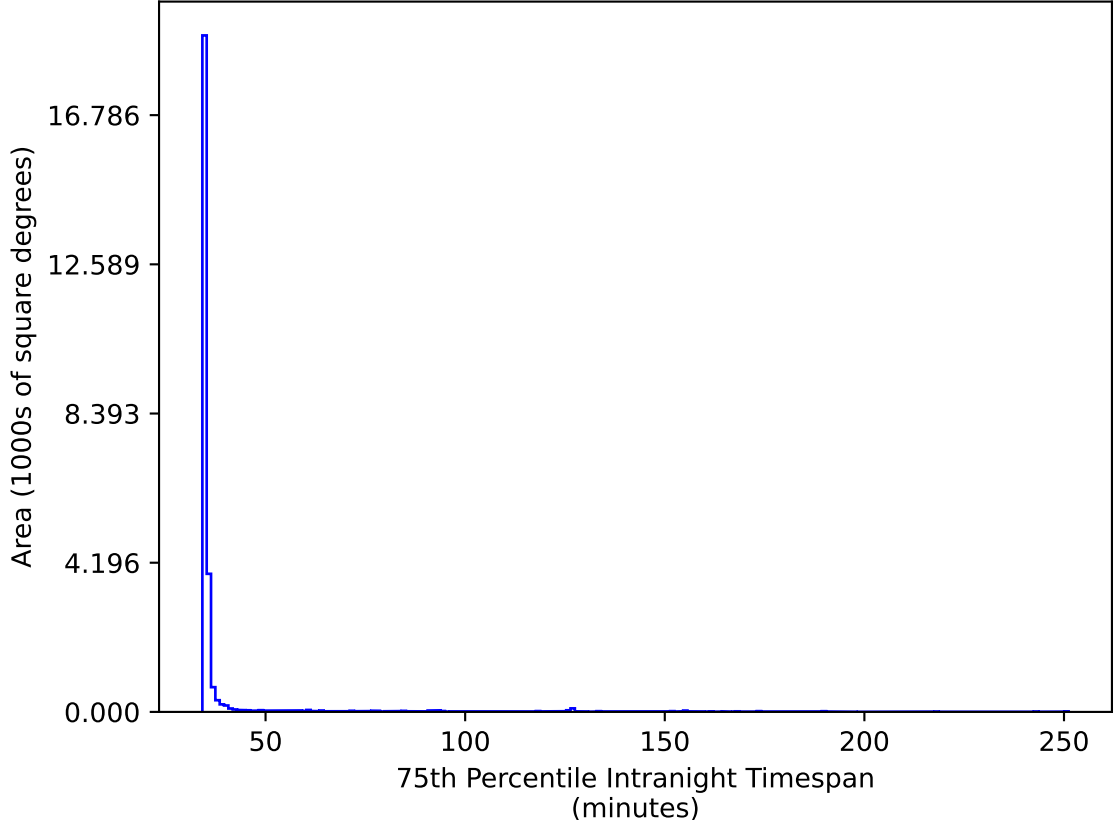
too_elab_r256_d2_gz_v3.4_10yrs All sky gr bands: 75th Percentile Intranight Timespan
