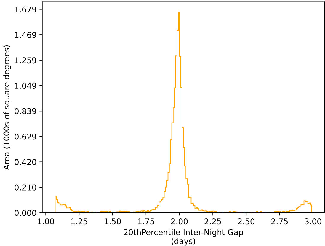
too_elab_r256_d2_gz_v3.4_10yrs WFD r band: 20thPercentile Inter-Night Gap
