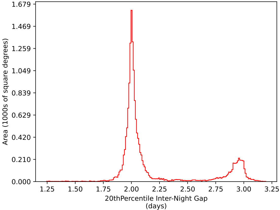
too_elab_r256_d2_gz_v3.4_10yrs WFD i band: 20thPercentile Inter-Night Gap
