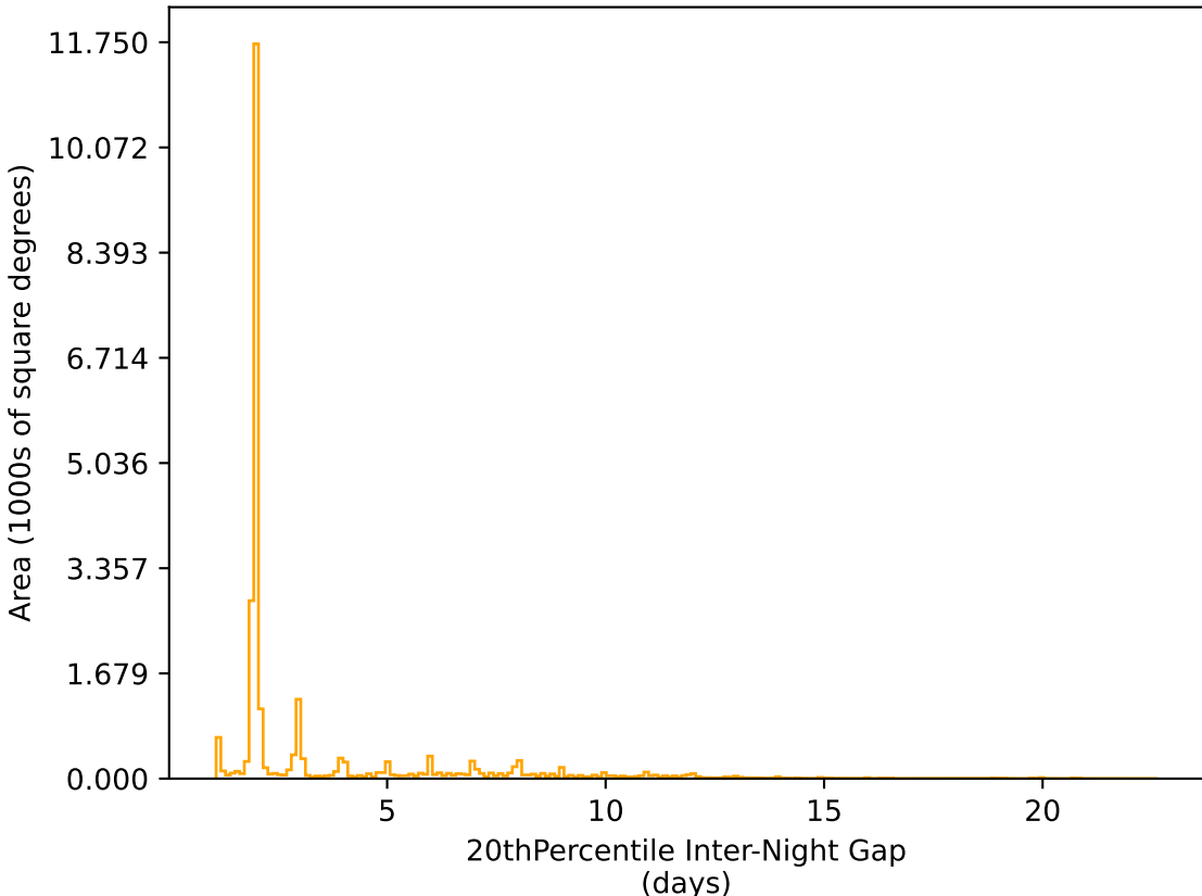
too_elab_r256_d2_gz_v3.4_10yrs All sky r band: 20thPercentile Inter-Night Gap
