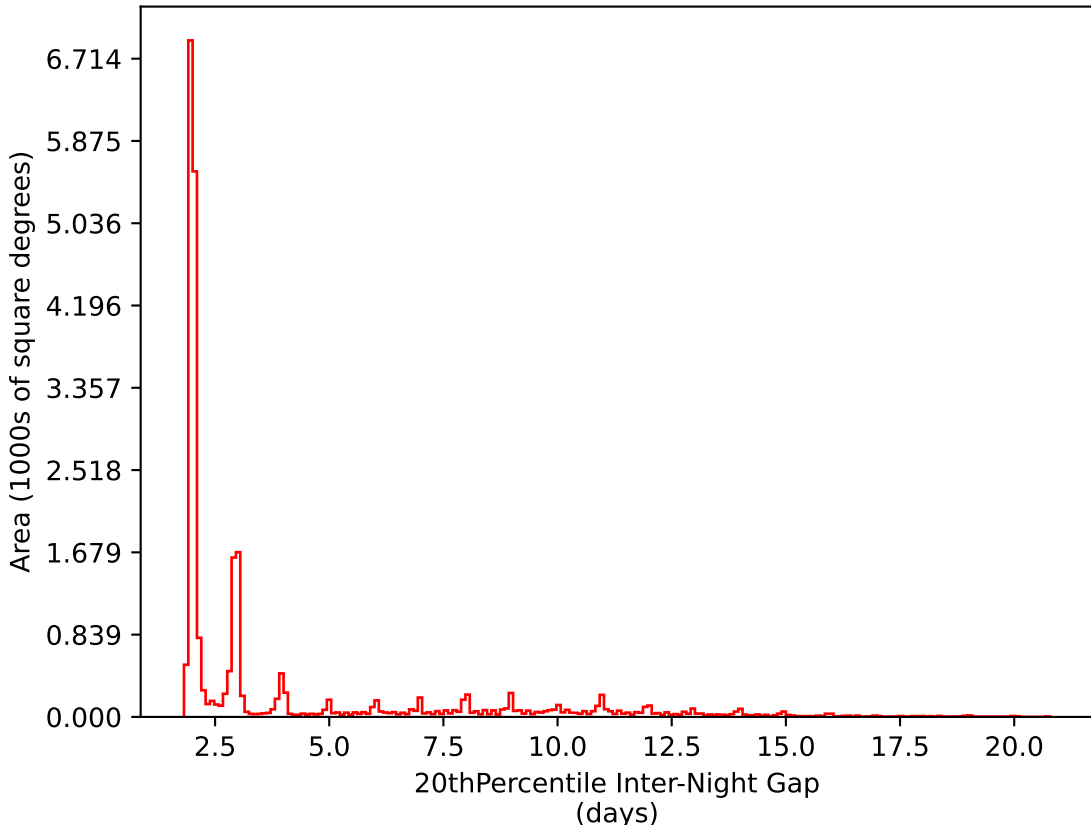
too_elab_r256_d2_gz_v3.4_10yrs All sky i band: 20thPercentile Inter-Night Gap
