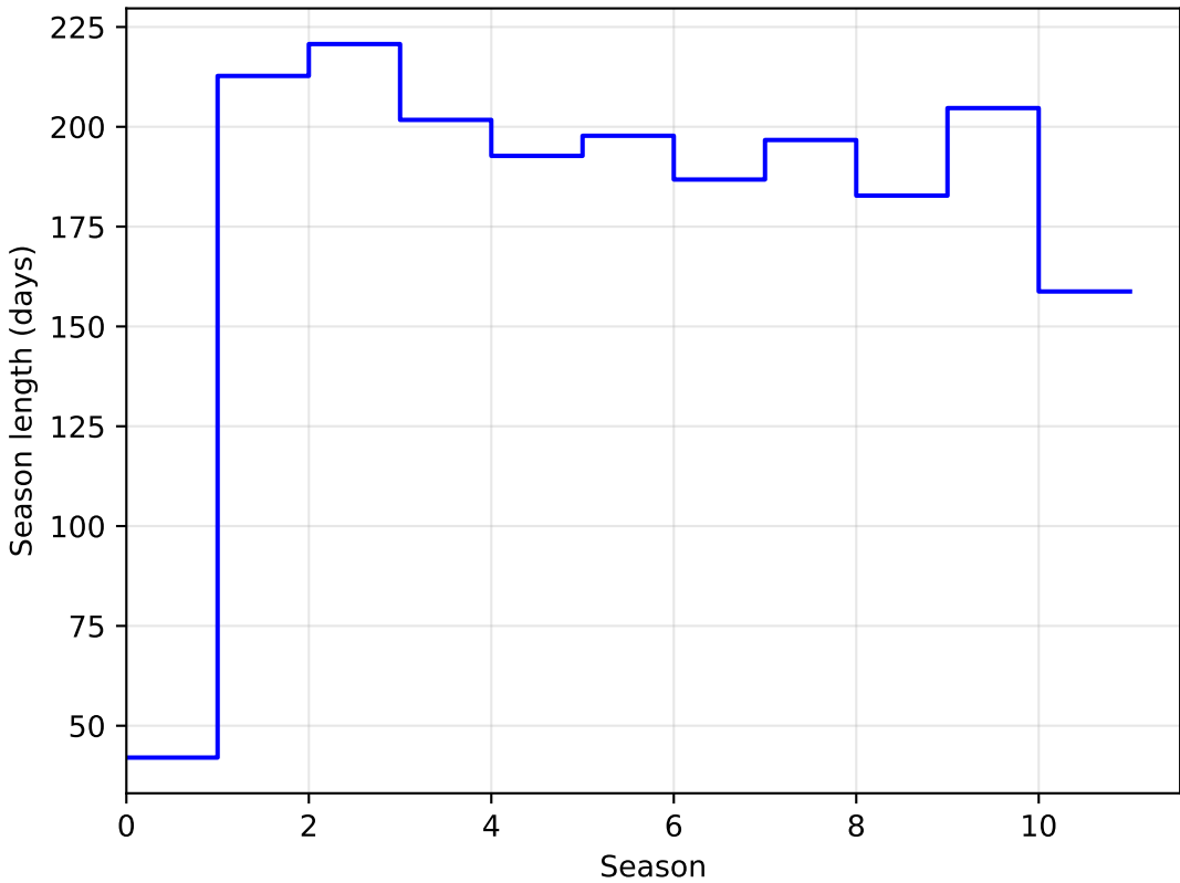
too_elab_r256_d2_gz_v3.4_10yrs DD: COSMOS all bands: SeasonLength
