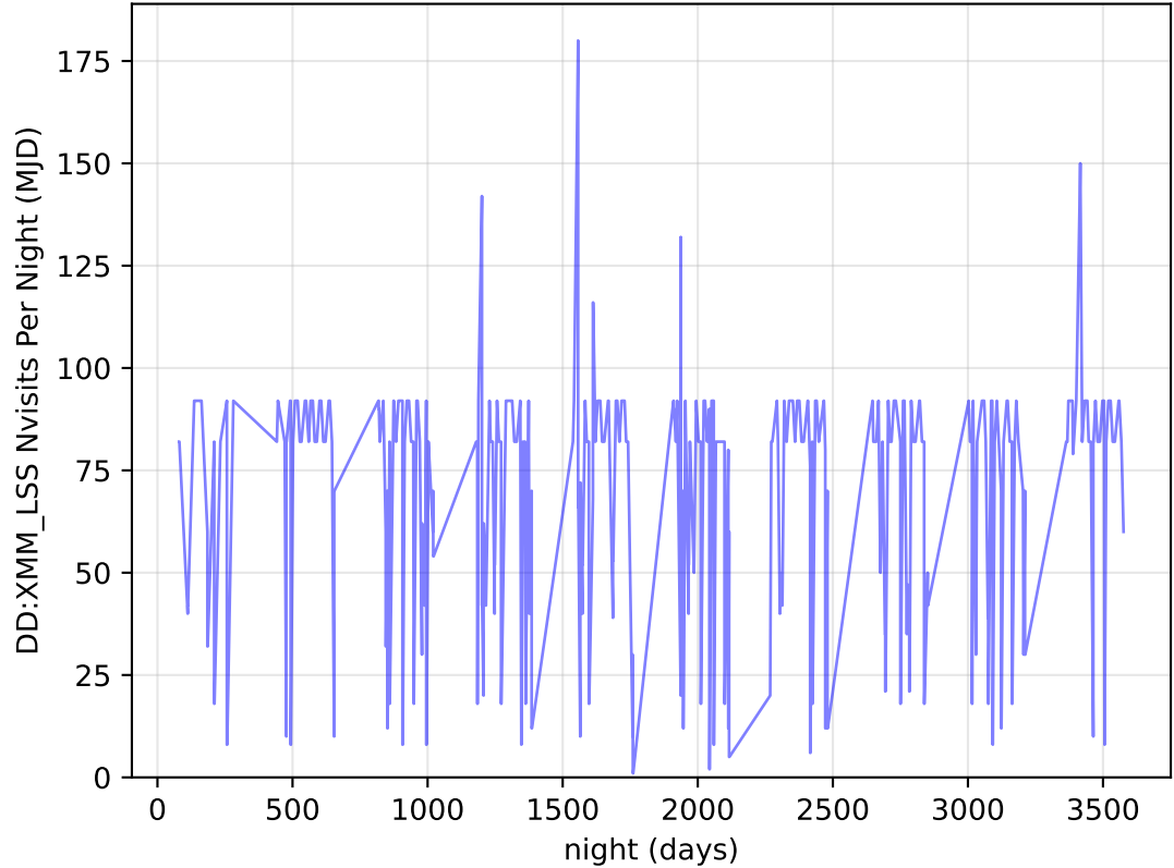
too_elab_r256_d2_gz_v3.4_10yrs all bands: DD:XMM_LSS Nvisits Per Night
