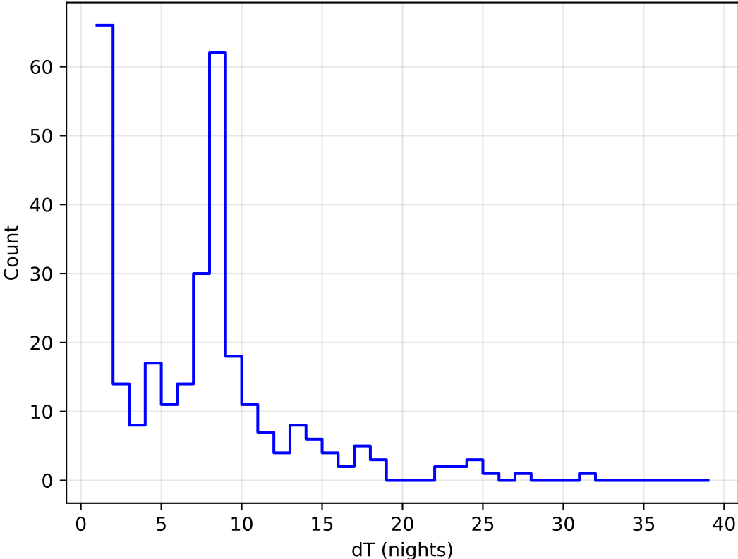
too_elab_r256_d2_gz_v3.4_10yrs all bands: DD:XMM_LSS Delta Nights Histogram
