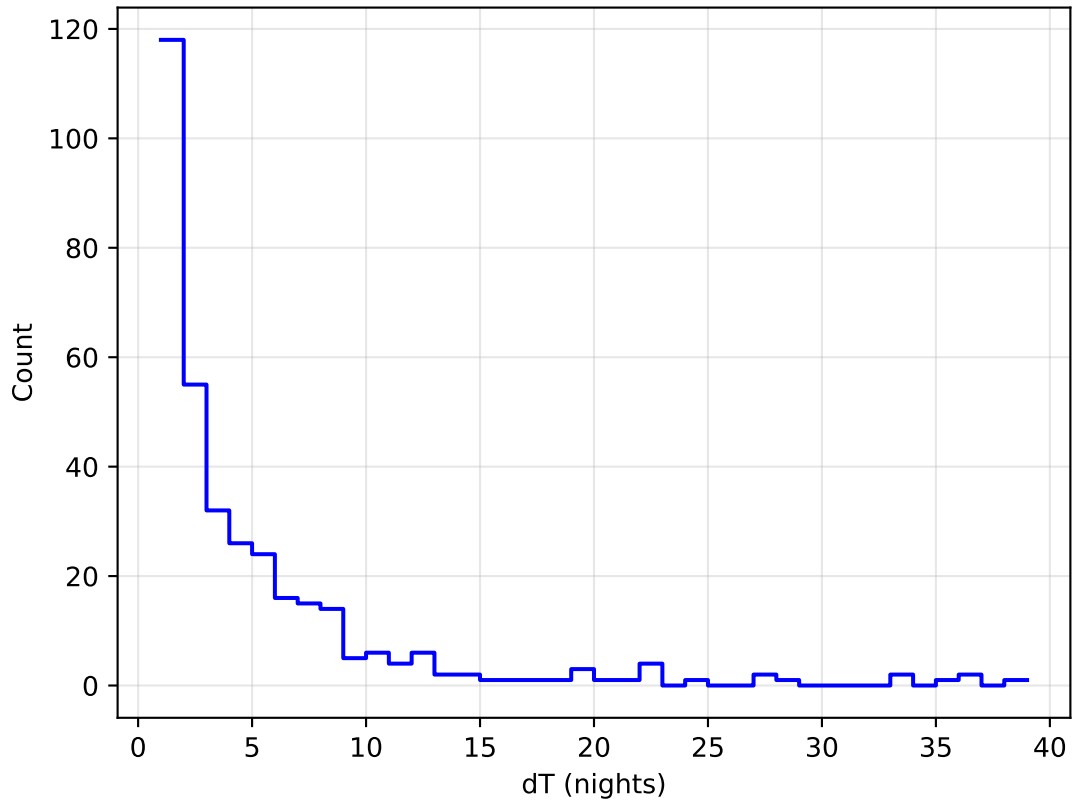
too_elab_r256_d2_gz_v3.4_10yrs all bands: DD:WFD Delta Nights Histogram
