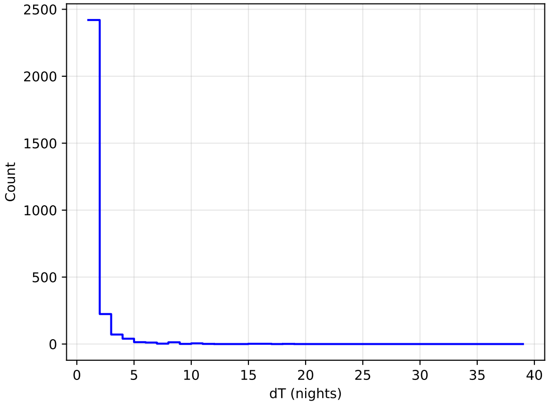
too_elab_r256_d2_gz_v3.4_10yrs all bands: DD:WFD Delta Nights Histogram
