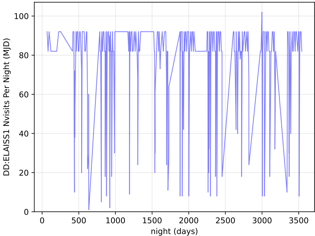
too_elab_r256_d2_gz_v3.4_10yrs all bands: DD:ELAISS1 Nvisits Per Night
