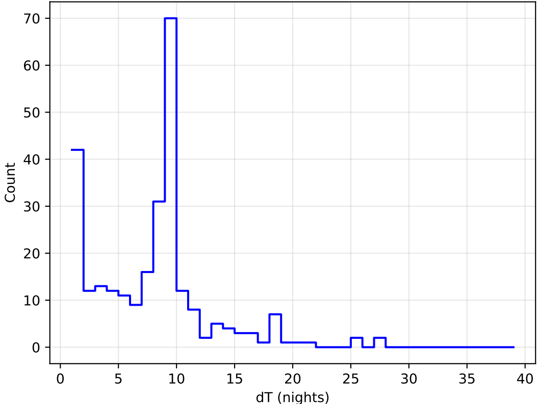
too_elab_r256_d2_gz_v3.4_10yrs all bands: DD:ELAISS1 Delta Nights Histogram
