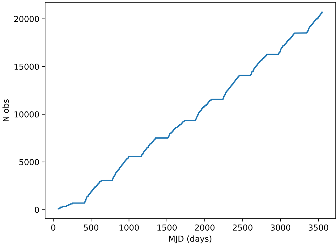
too_elab_r256_d2_gz_v3.4_10yrs all bands: DD:ELAISS1 Cumulative NVisits
