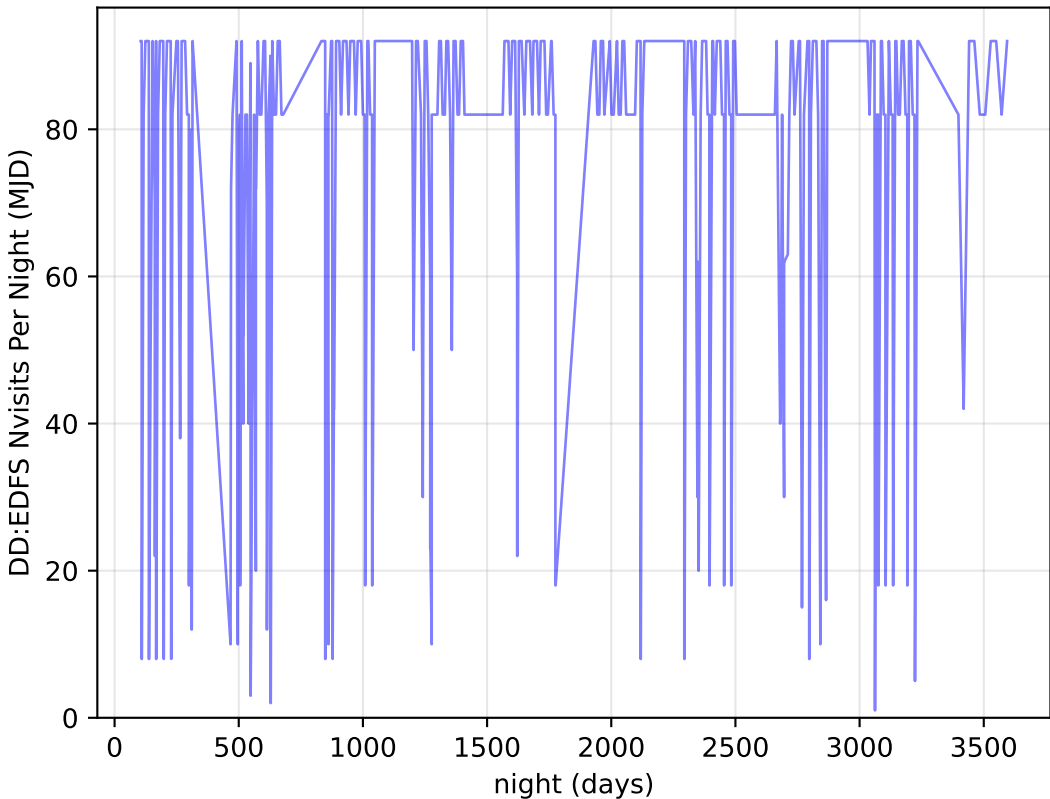
too_elab_r256_d2_gz_v3.4_10yrs all bands: DD:EDFS Nvisits Per Night
