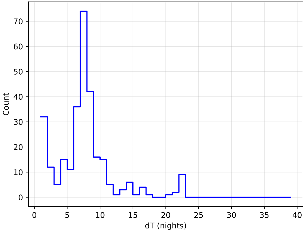
too_elab_r256_d2_gz_v3.4_10yrs all bands: DD:EDFS Delta Nights Histogram
