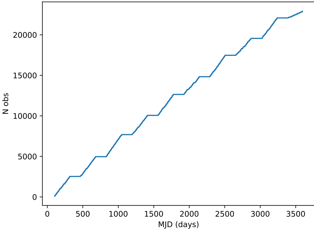
too_elab_r256_d2_gz_v3.4_10yrs all bands: DD:EDFS Cumulative NVisits
