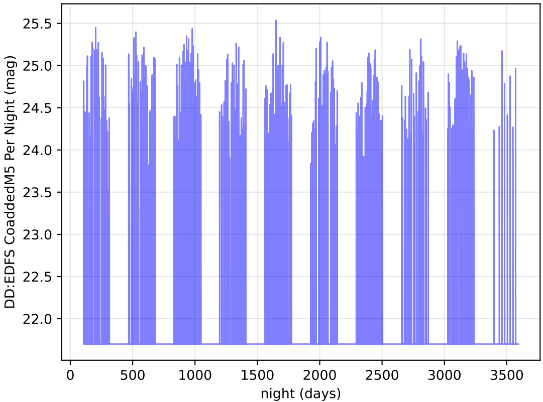
too_elab_r256_d2_gz_v3.4_10yrs z band: DD:EDFS CoaddedM5 Per Night
