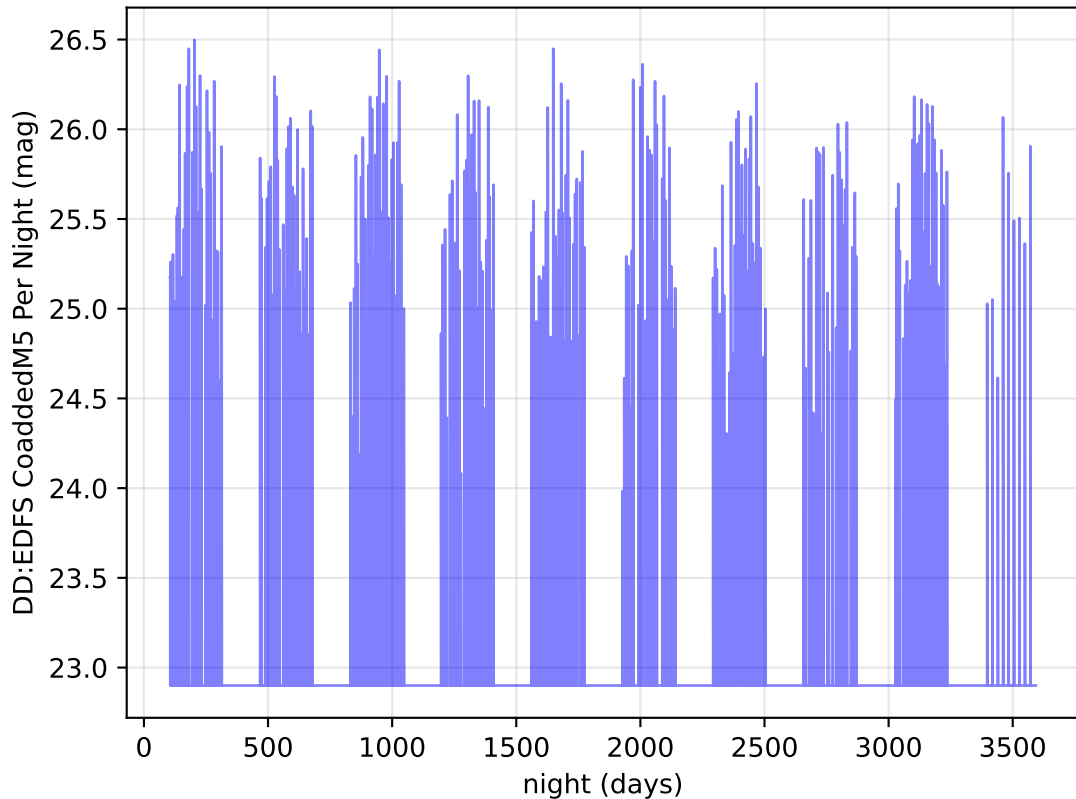
too_elab_r256_d2_gz_v3.4_10yrs r band: DD:EDFS CoaddedM5 Per Night
