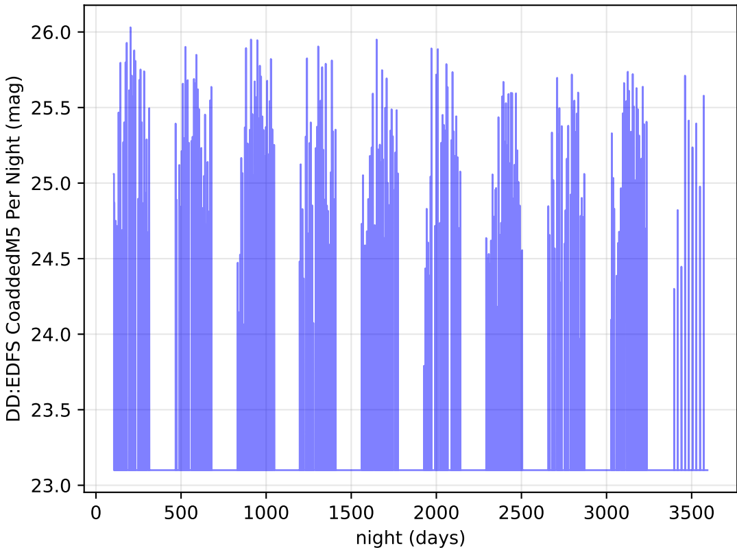
too_elab_r256_d2_gz_v3.4_10yrs i band: DD:EDFS CoaddedM5 Per Night
