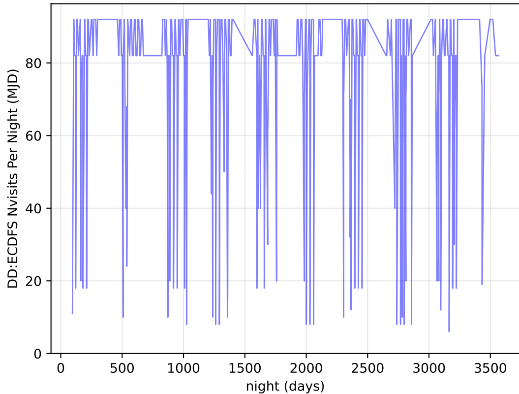
too_elab_r256_d2_gz_v3.4_10yrs all bands: DD:ECDFS Nvisits Per Night
