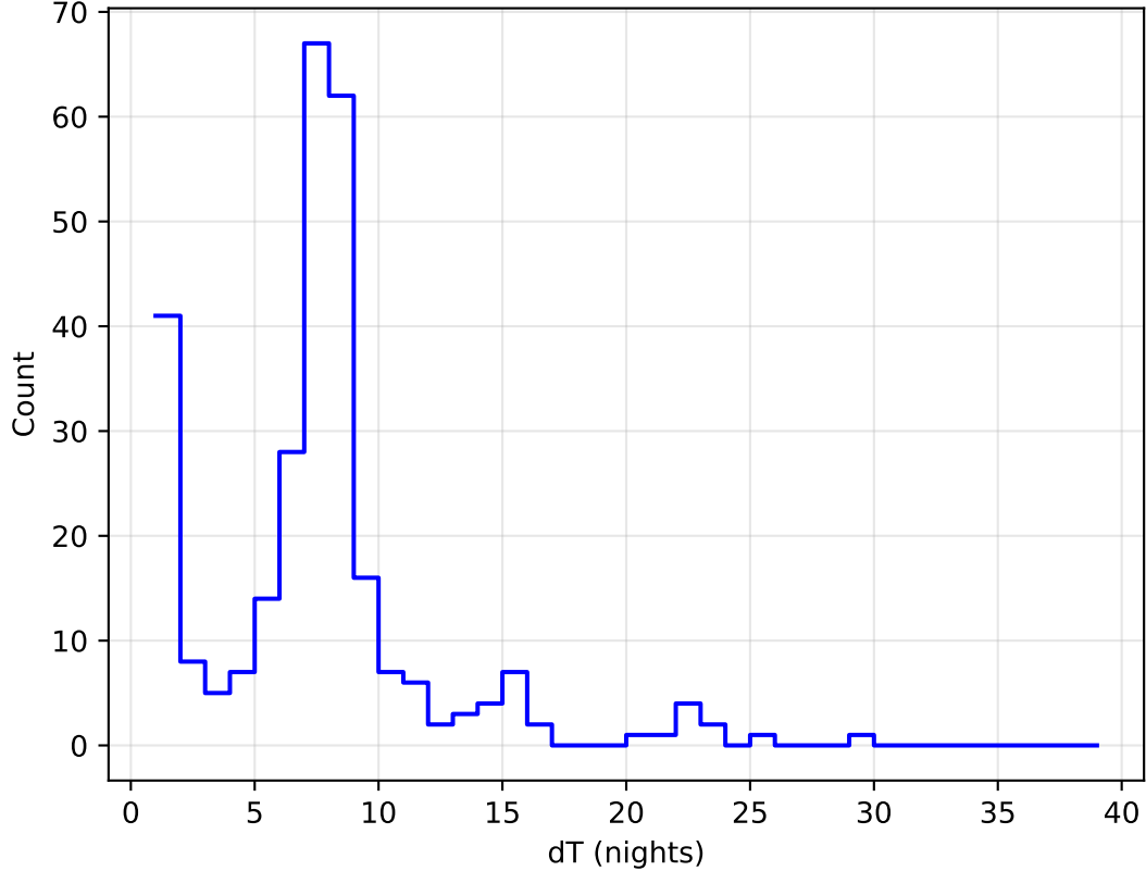
too_elab_r256_d2_gz_v3.4_10yrs all bands: DD:ECDFS Delta Nights Histogram
