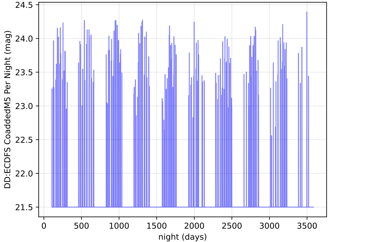
too_elab_r256_d2_gz_v3.4_10yrs y band: DD:ECDFS CoaddedM5 Per Night
