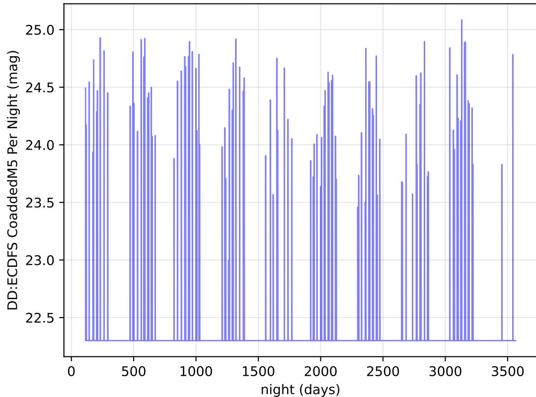
too_elab_r256_d2_gz_v3.4_10yrs u band: DD:ECDFS CoaddedM5 Per Night
