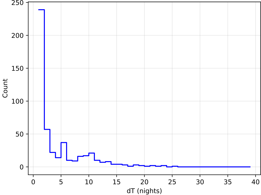
too_elab_r256_d2_gz_v3.4_10yrs all bands: DD: COSMOS Delta Nights Histogram
