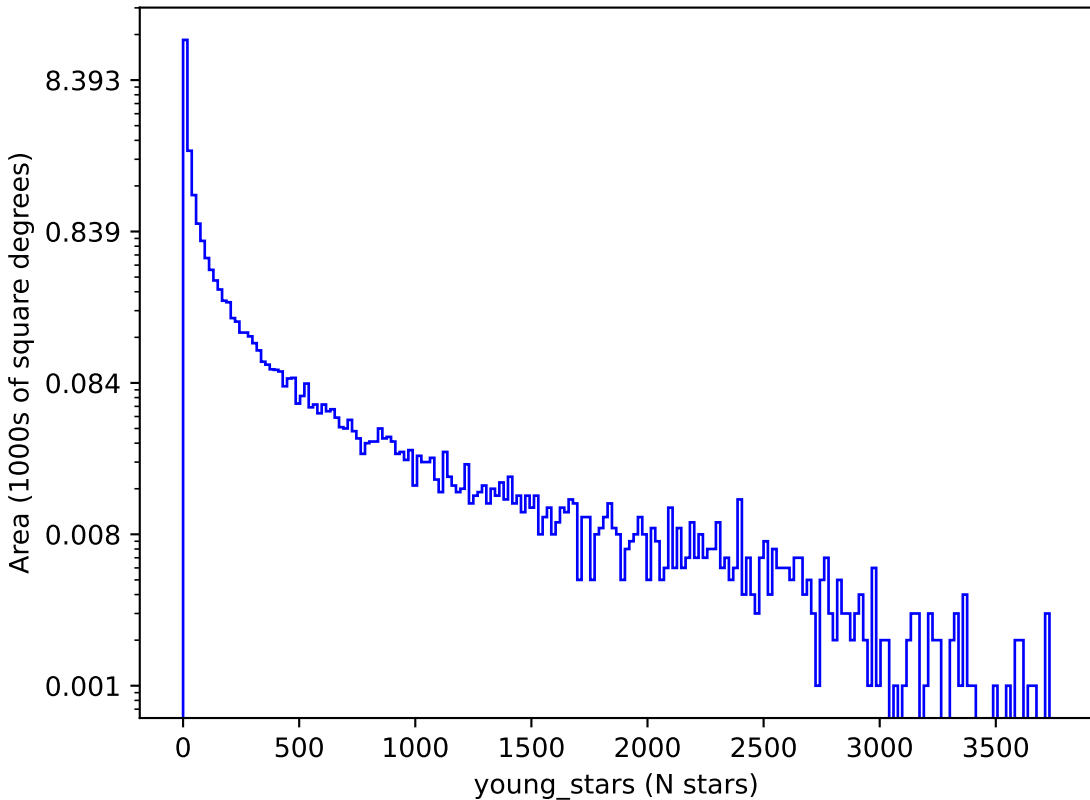
too_elab_r256_d2_griz_v3.4_10yrs : young_stars
