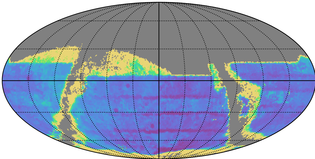
too_elab_r256_d2_griz_v3.4_10yrs : TDC_accuracy
