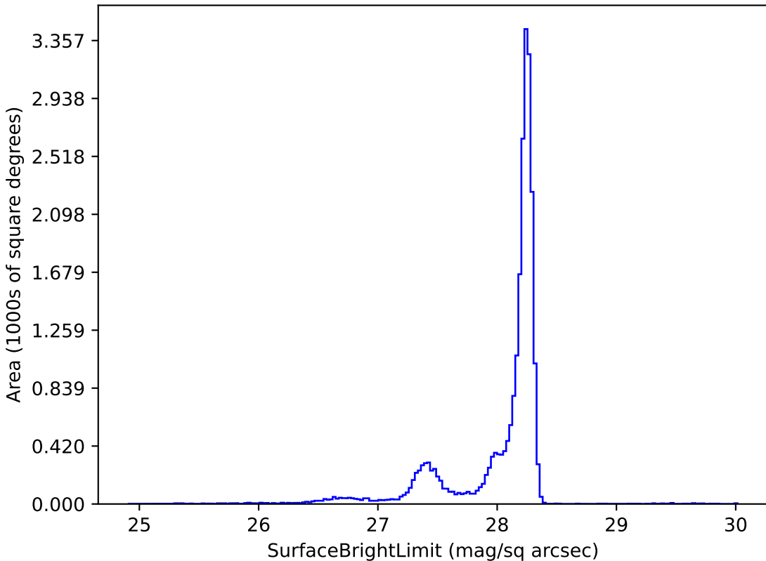
too_elab_r256_d2_griz_v3.4_10yrs y: SurfaceBrightLimit
