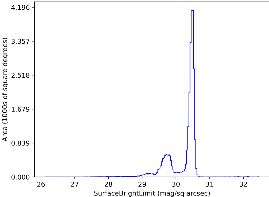
too_elab_r256_d2_griz_v3.4_10yrs r: SurfaceBrightLimit
