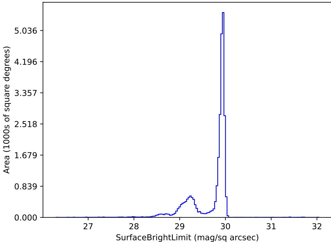
too_elab_r256_d2_griz_v3.4_10yrs i: SurfaceBrightLimit
