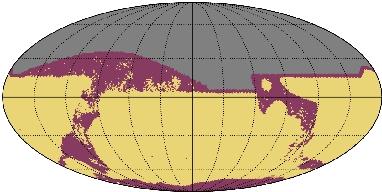
too_elab_r256_d2_griz_v3.4_10yrs : RapidRevisits
