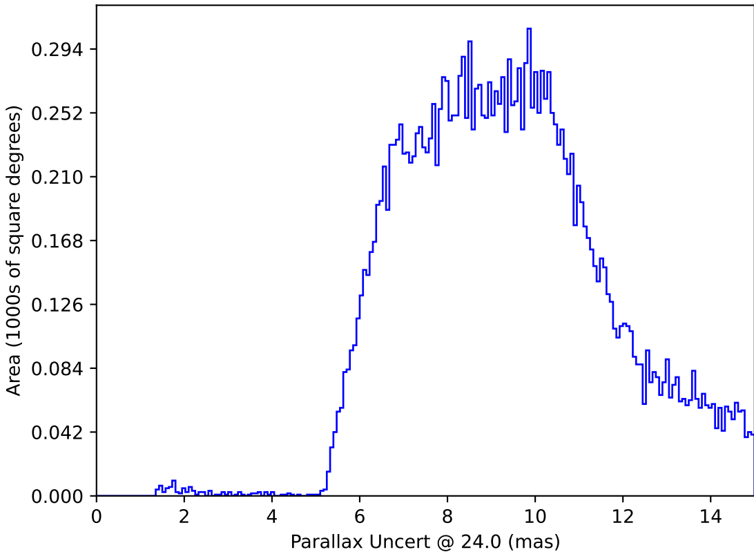
too_elab_r256_d2_griz_v3.4_10yrs : Parallax Uncert @ 24.0
