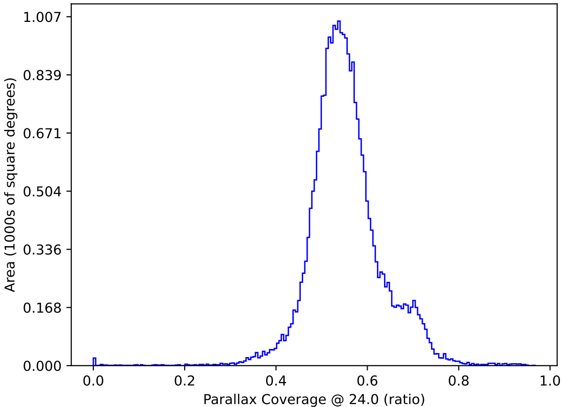
too_elab_r256_d2_griz_v3.4_10yrs : Parallax Coverage @ 24.0
