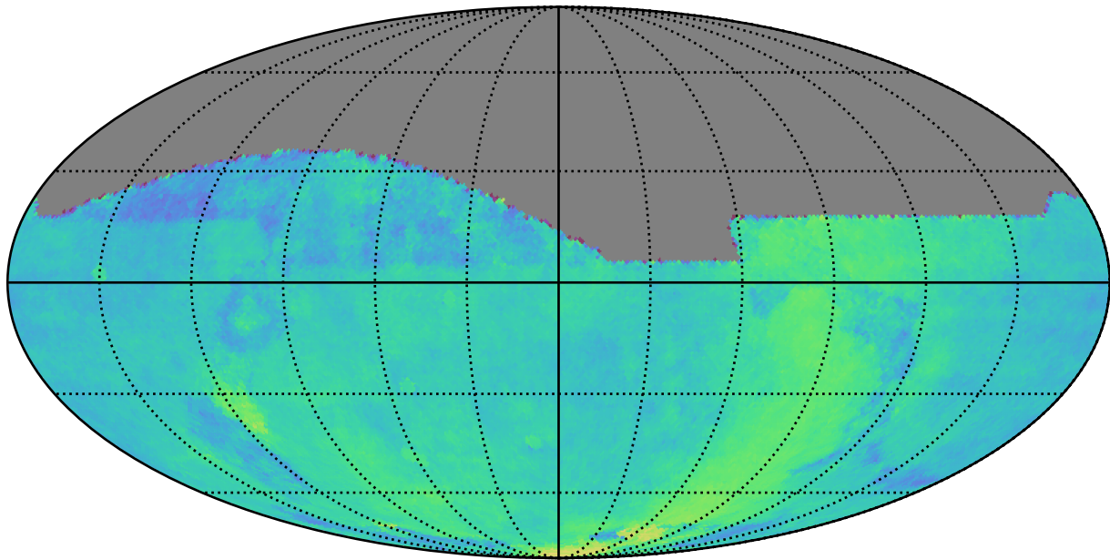
too_elab_r256_d2_griz_v3.4_10yrs : Parallax Coverage @ 22.4
