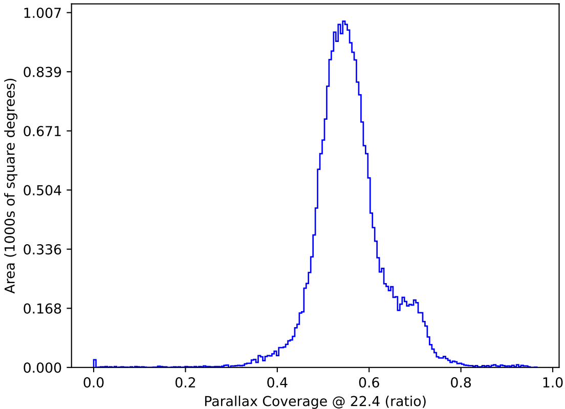
too_elab_r256_d2_griz_v3.4_10yrs : Parallax Coverage @ 22.4
