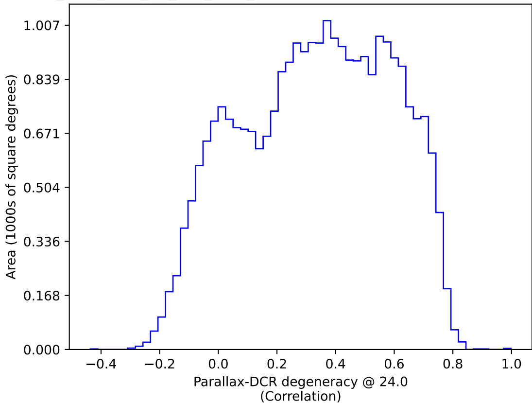
too_elab_r256_d2_griz_v3.4_10yrs : Parallax-DCR degeneracy @ 24.0
