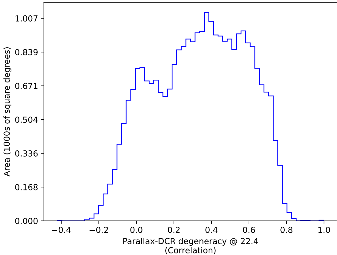
too_elab_r256_d2_griz_v3.4_10yrs : Parallax-DCR degeneracy @ 22.4
