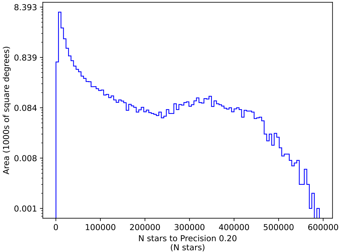
too_elab_r256_d2_griz_v3.4_10yrs y: N stars to Precision 0.20
