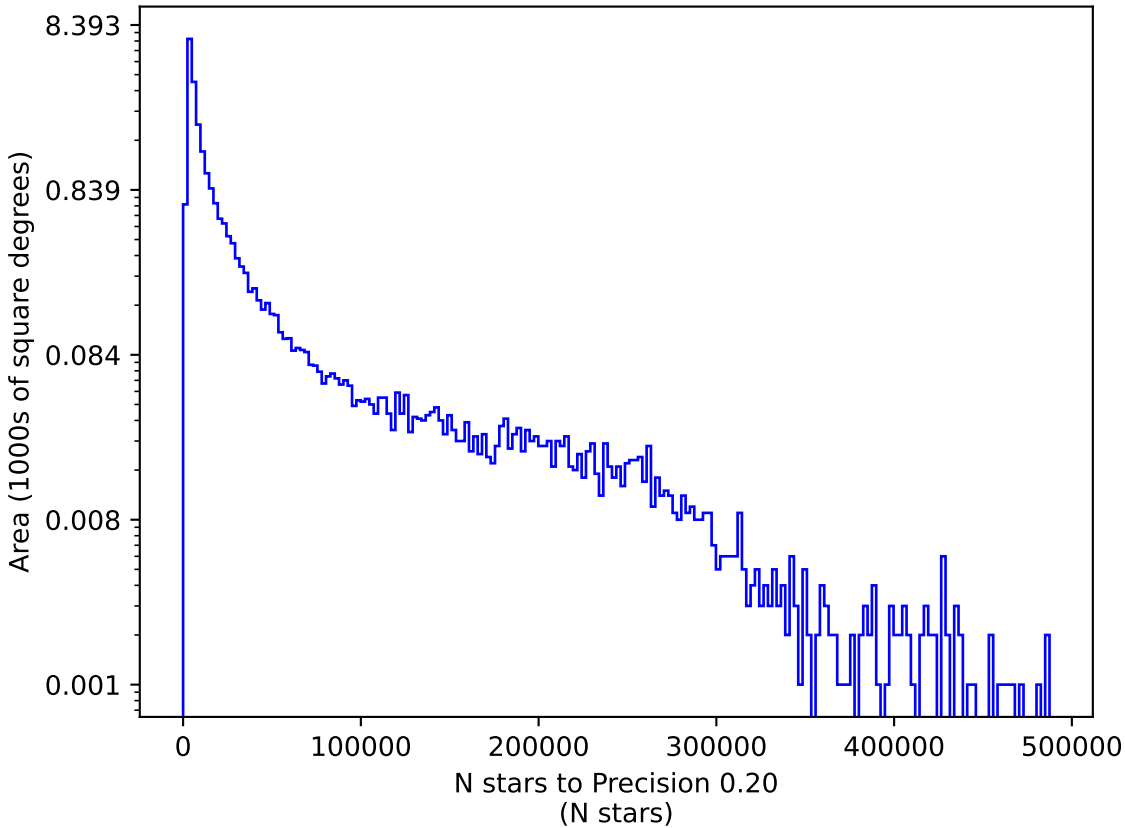
too_elab_r256_d2_griz_v3.4_10yrs u: N stars to Precision 0.20
