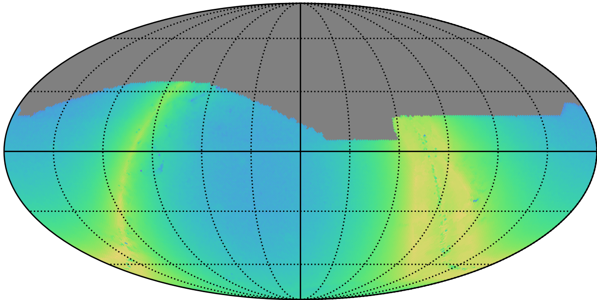
too_elab_r256_d2_griz_v3.4_10yrs r: N stars to Precision 0.20
