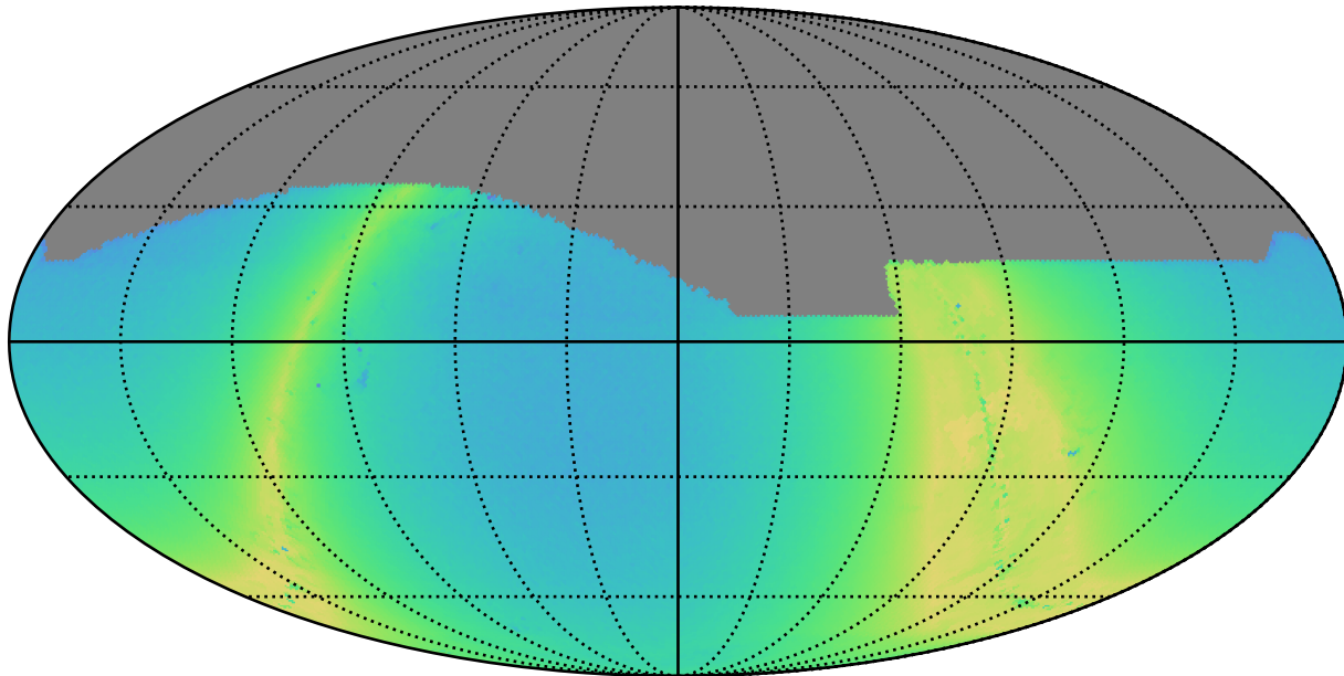
too_elab_r256_d2_griz_v3.4_10yrs i: N stars to Precision 0.20
