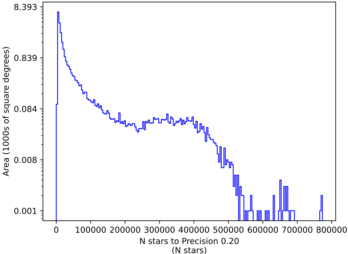
too_elab_r256_d2_griz_v3.4_10yrs g: N stars to Precision 0.20
