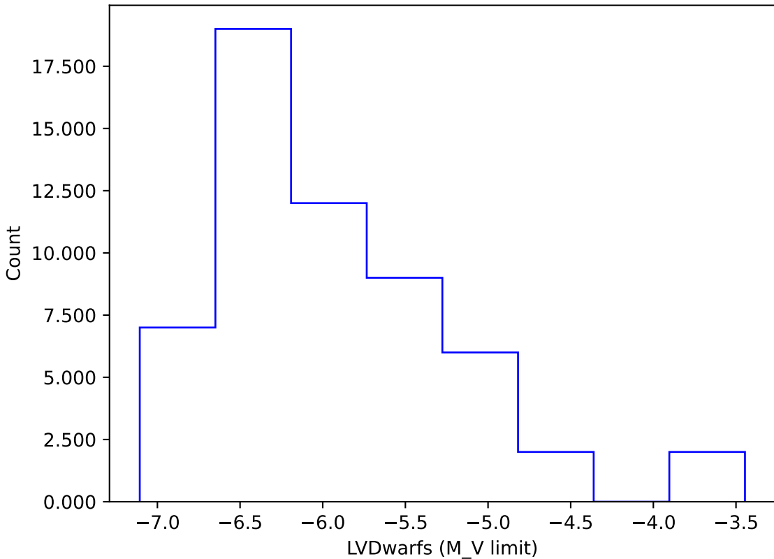
too_elab_r256_d2_griz_v3.4_10yrs gi: LVDwarfs
