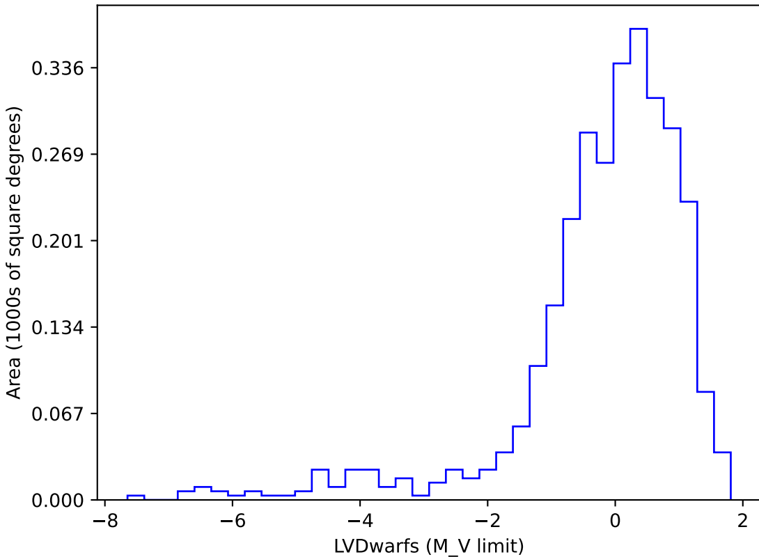
too_elab_r256_d2_griz_v3.4_10yrs gi SCP: LVDwarfs
