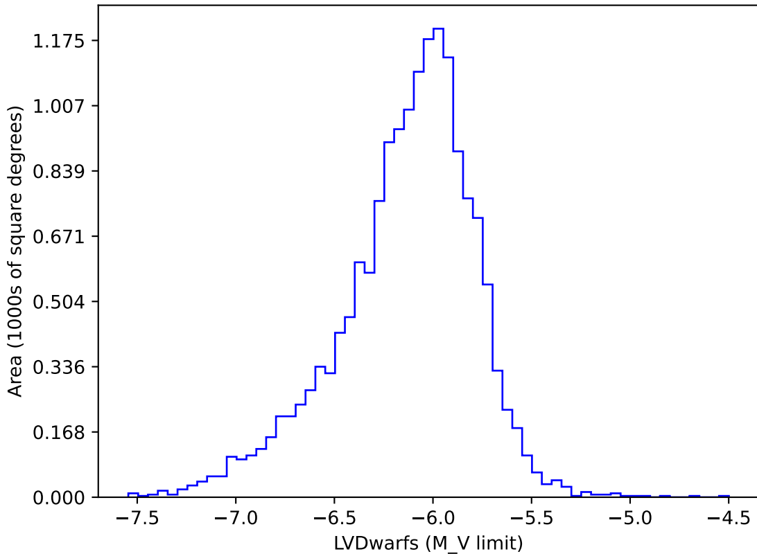
too_elab_r256_d2_griz_v3.4_10yrs gi: LVDwarfs
