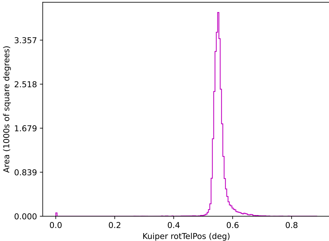
too_elab_r256_d2_griz_v3.4_10yrs z: Kuiper rotTelPos
